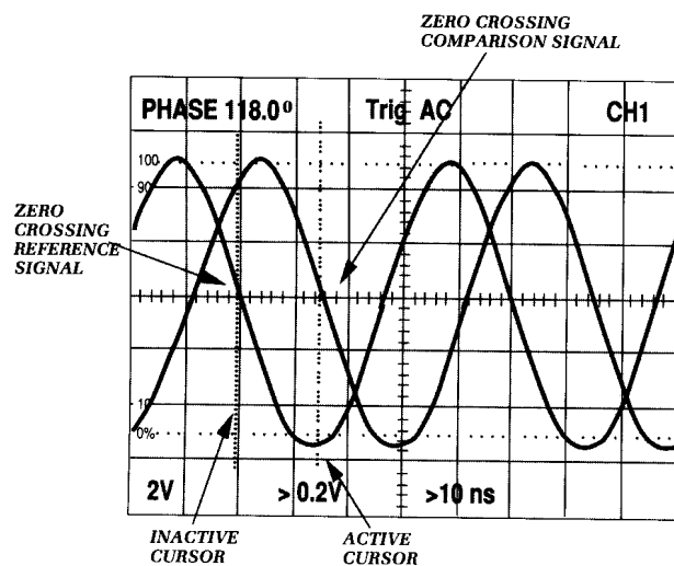
Figure 3-9: Phase Difference Measurement
