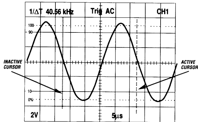
Figure 3-6: Frequency Measurement
