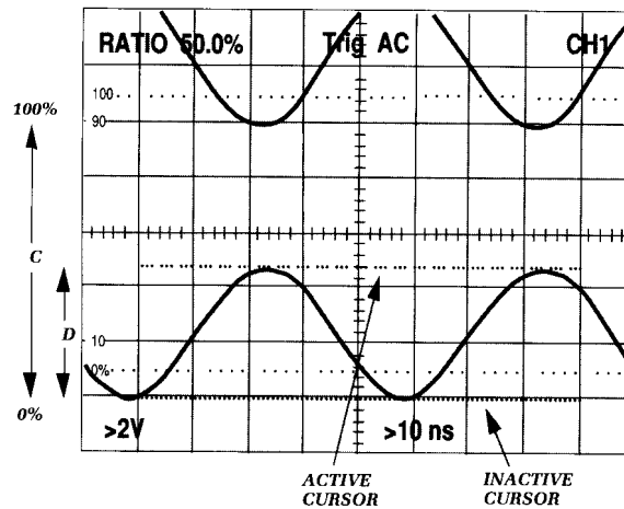
Figure 3-11: Percentage Modulation.
