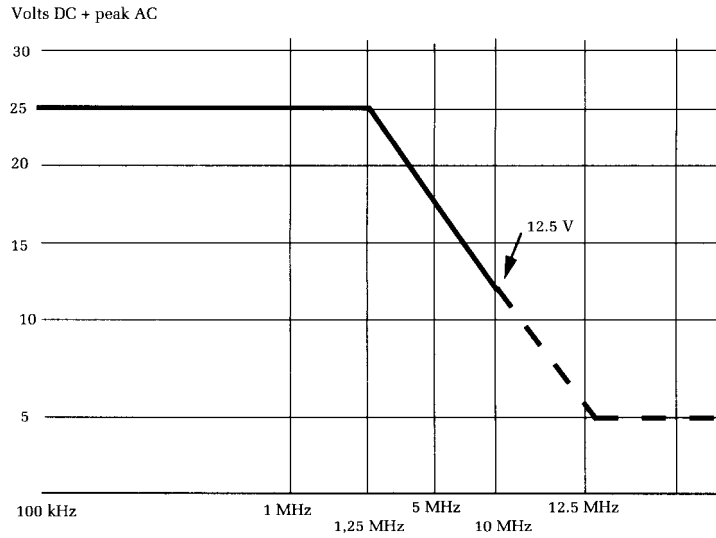
Figure B-1: Maximum Input Voltage Versus Frequency Derating Curve for the EXT CLK Connector
