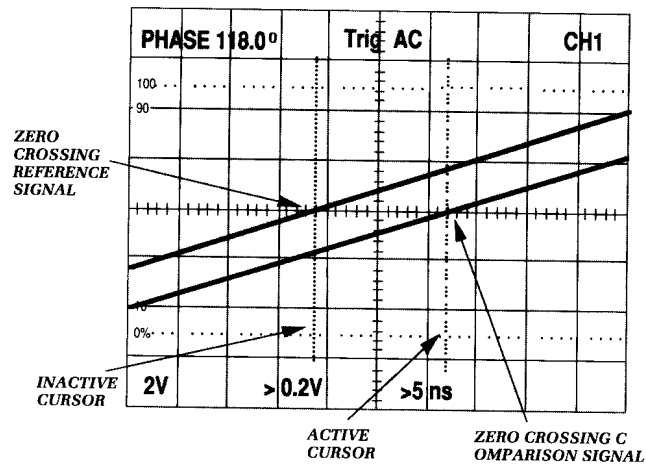
Figure 3-10: Small-angle Phase Difference Measurement
