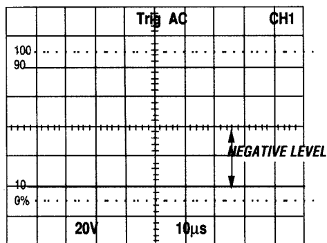
(B) CH 2 DISPLAY WITH 2 DIVISIONS OF NEGATIVE OFFSET
