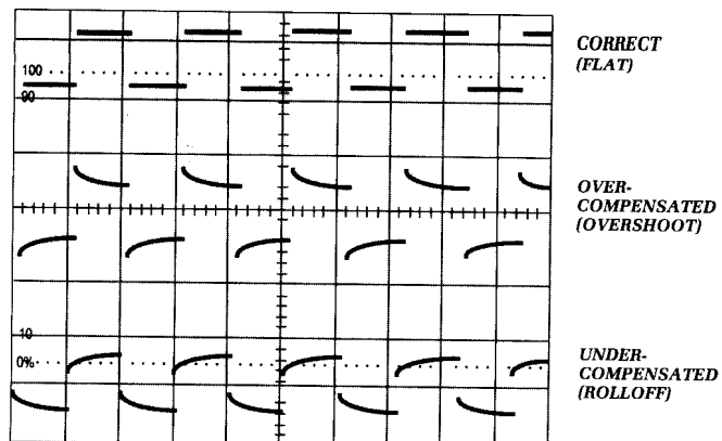
Figure 2-1: Probe Compensation
