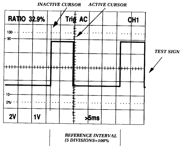
Figure 3-8: Time Ratio Measurement
