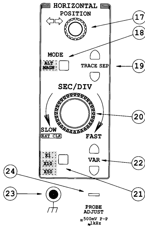
Figure 5-3: Horizontal Controls and Switches
