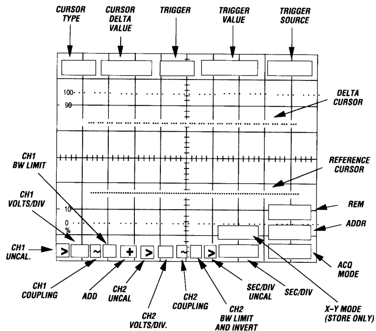
Figure 5-10: CRT Readout Display Fields
