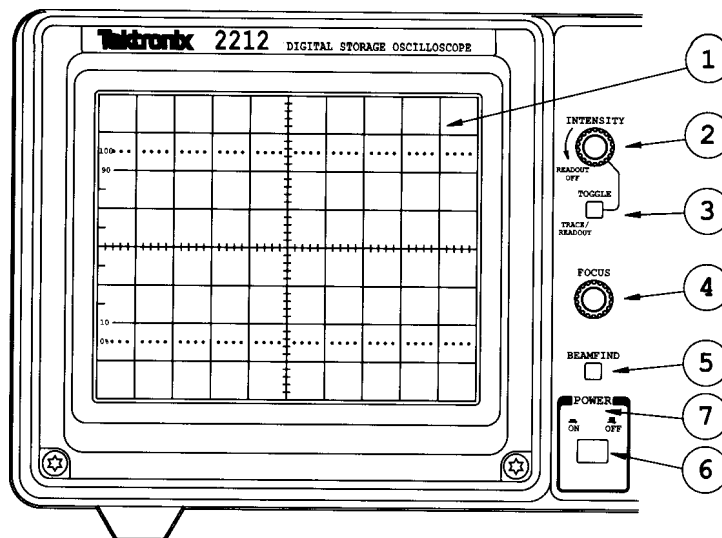
Figure 5-1: Power and Display Controls and Power-on Indicator
