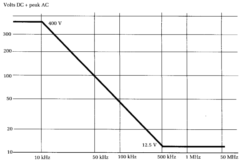
Figure B-2: Maximum Voltage Versus Frequency Derating Curve for the CH1 OR X, CH 2 OR Y, and EXT OR Z Connectors
