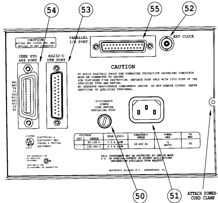
Figure 5-9 Rear Panel (Partial)
