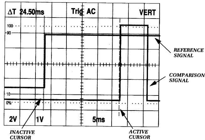
Figure 3-7: Time Difference Measurement between two Time-related Pulses
