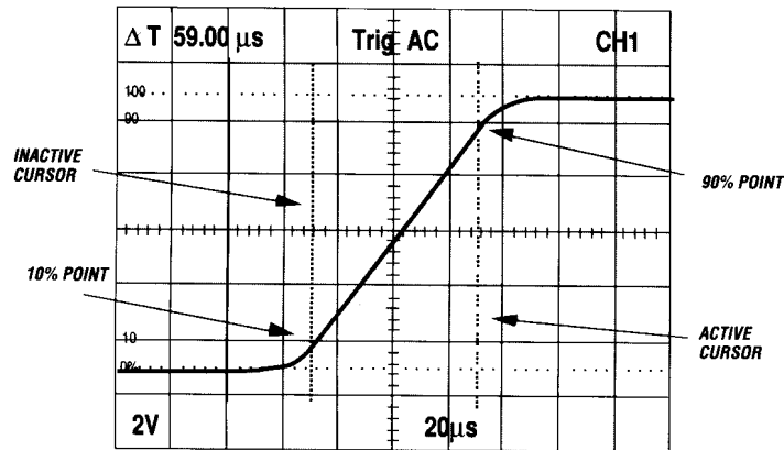
Figure 3-5: Rise Time Measurement
