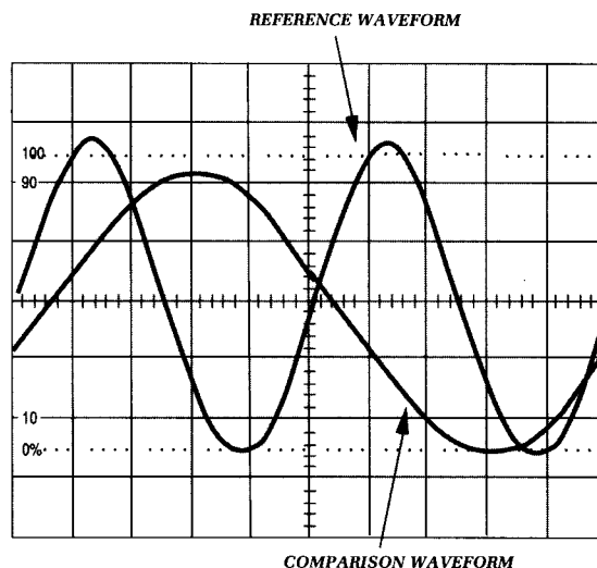
Figure 3-12: Waveform Comparison Measurement
