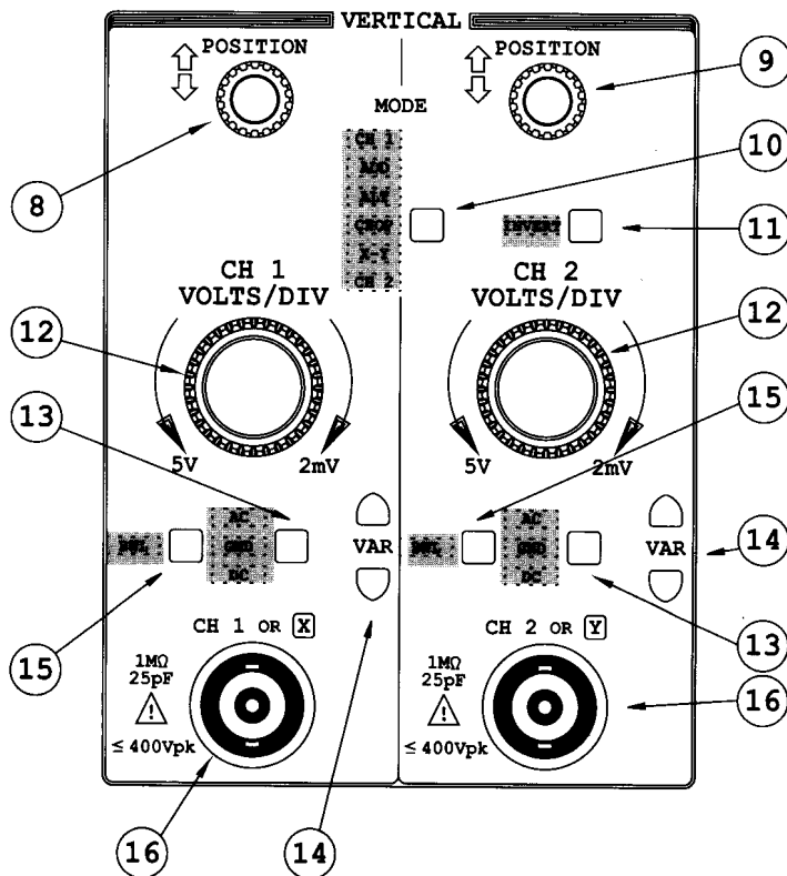
Figure 5-2: Vertical Controls and Connectors
