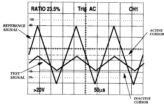
Figure 3-2: Voltage Ratios
