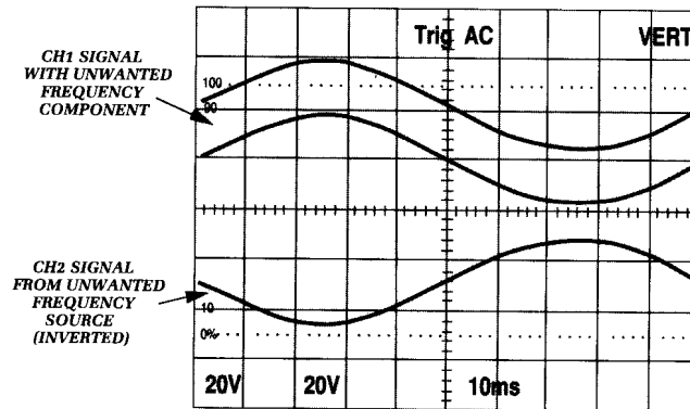
(A) CH1 AND CH2 SIGNALS
