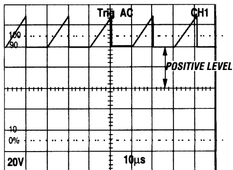
(A) CH 1 SIGNAL WITH 2 DIVISIONS OF POSITIVE DC LEVEL
